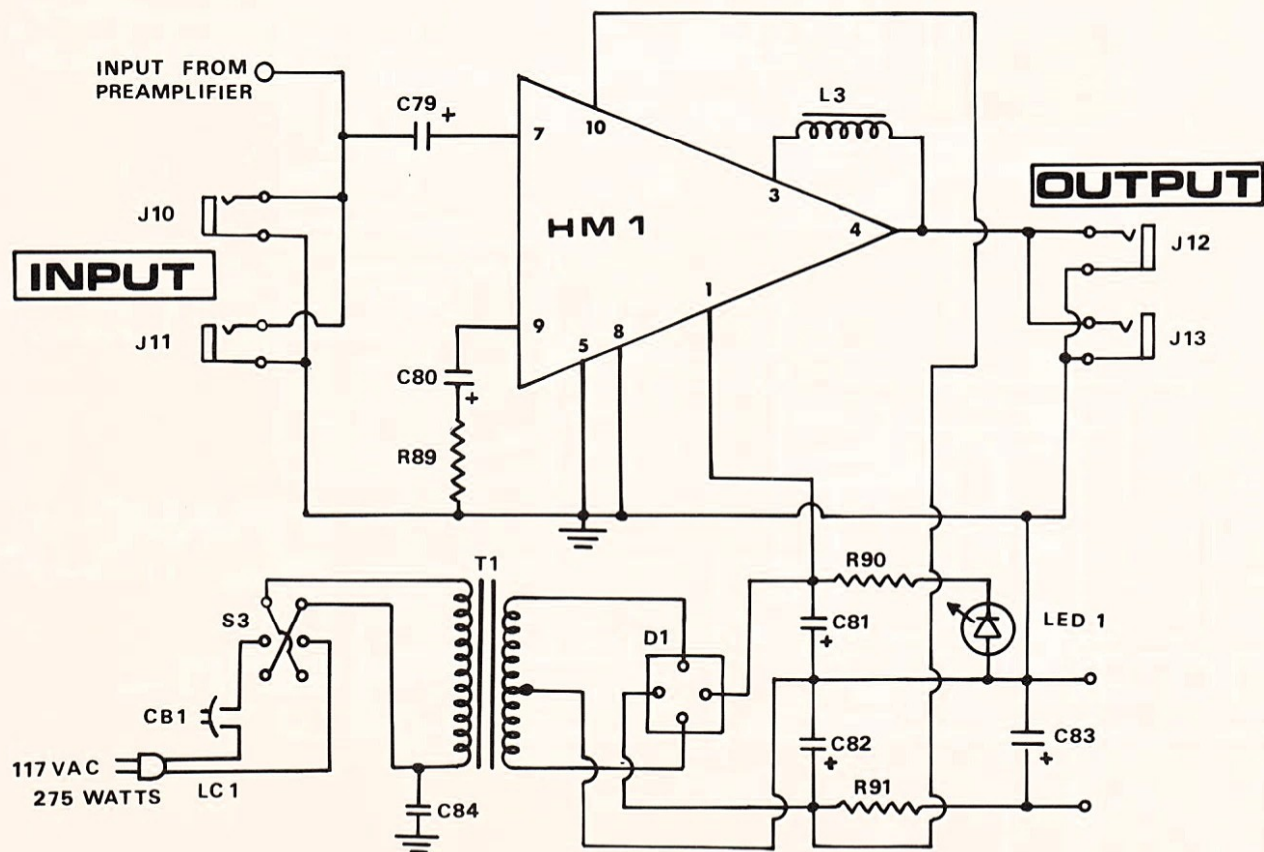
PCB 2- CIRCUIT BOARD POWER AMPLIFIER
